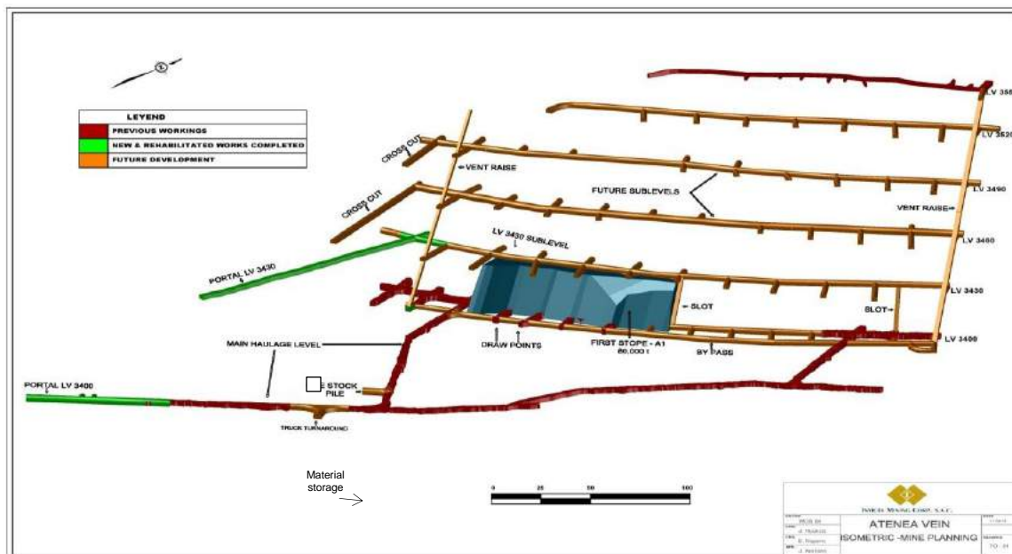
Figure 3 – Invicta Development Plan (3D – Oblique Long Section)
